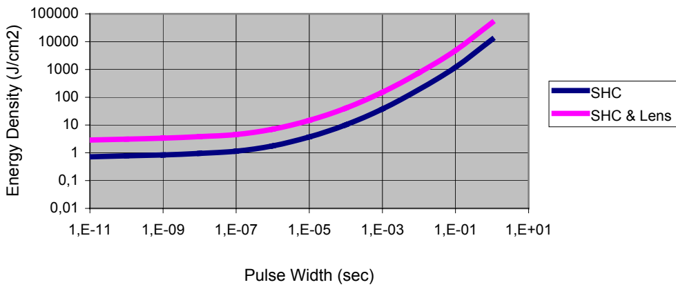
A30-D12-SHC-L vs A30-D12-SHC: Damage Thresholds
